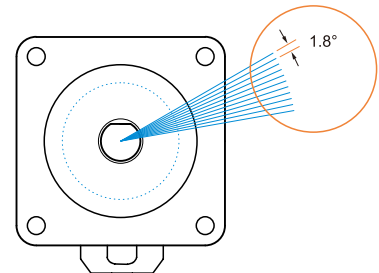
Schematic diagram of the step angle of a two-phase hybrid stepper motor.
